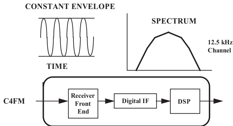
Figure 1-4: C4FM Demodulator
