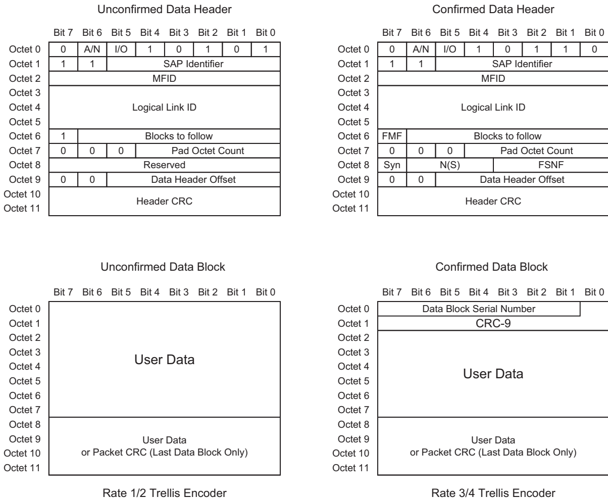
Figure 4-13: Unconfirmed and Confirmed Header and Data Blocks
