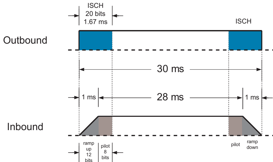
Figure 7-8: TDMA Transmission Format
