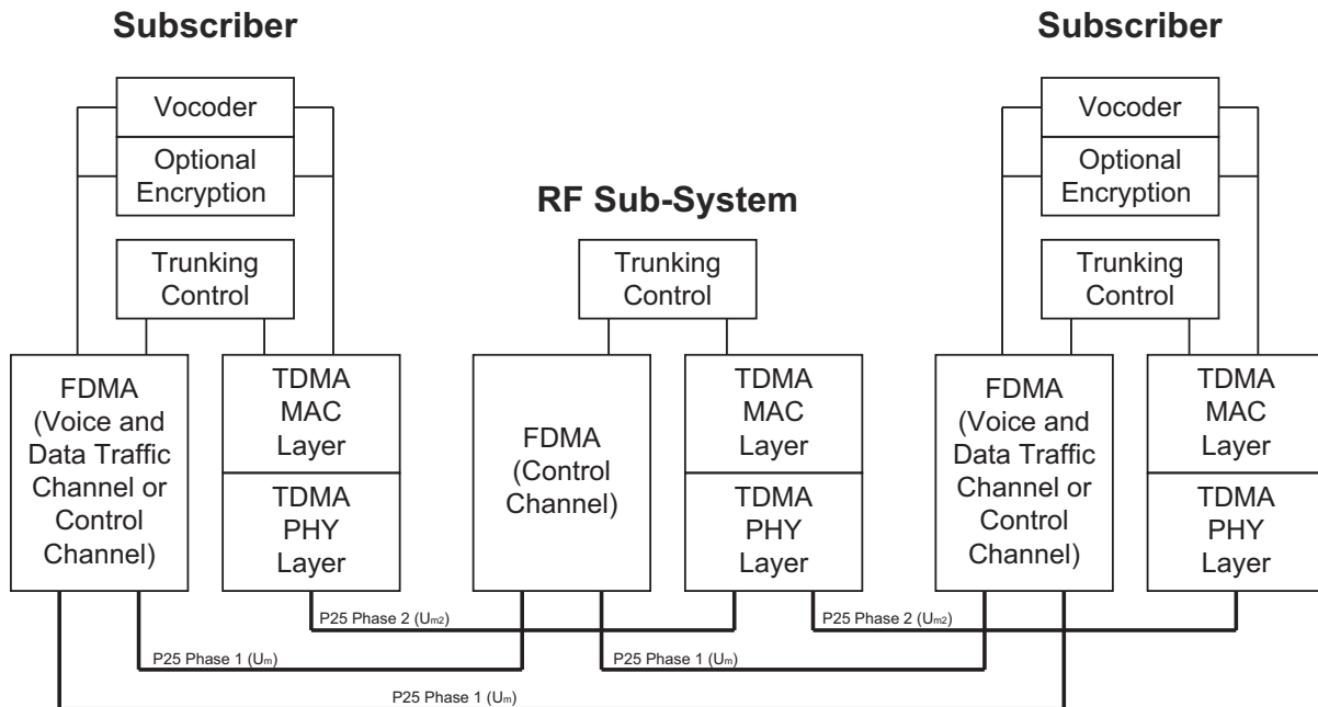
Figure 7-6: P25 Two-Slot TDMA Protocol Model
