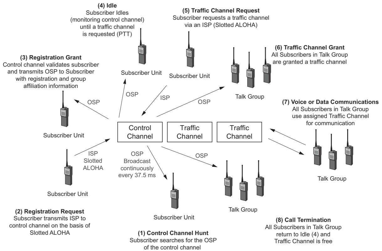
Figure 6-3: P25 Trunking System Operation
